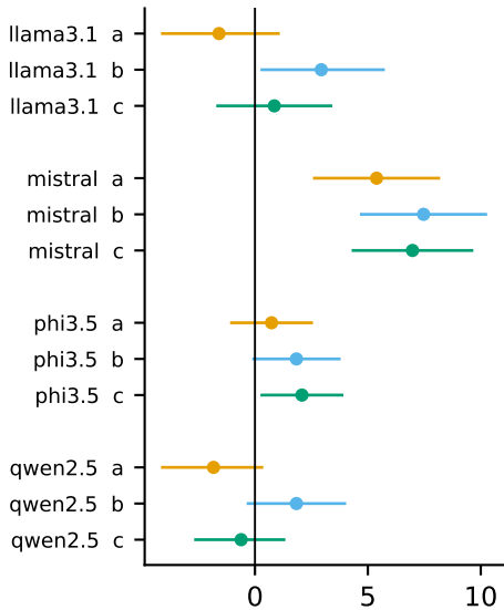
TruthfulQA delta
