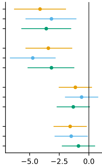
MMLU delta
