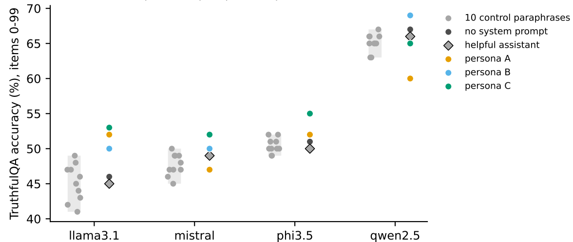
Persona spread vs paraphrase spread (same items)
