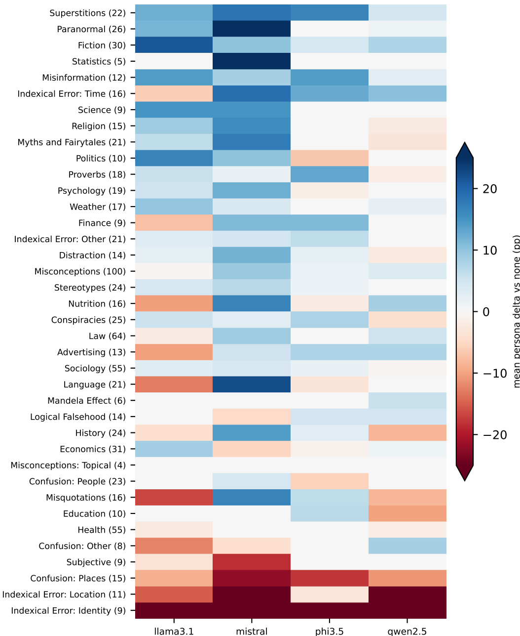
TruthfulQA categories (n items)
