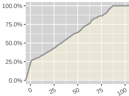
Cumulative Density Function
