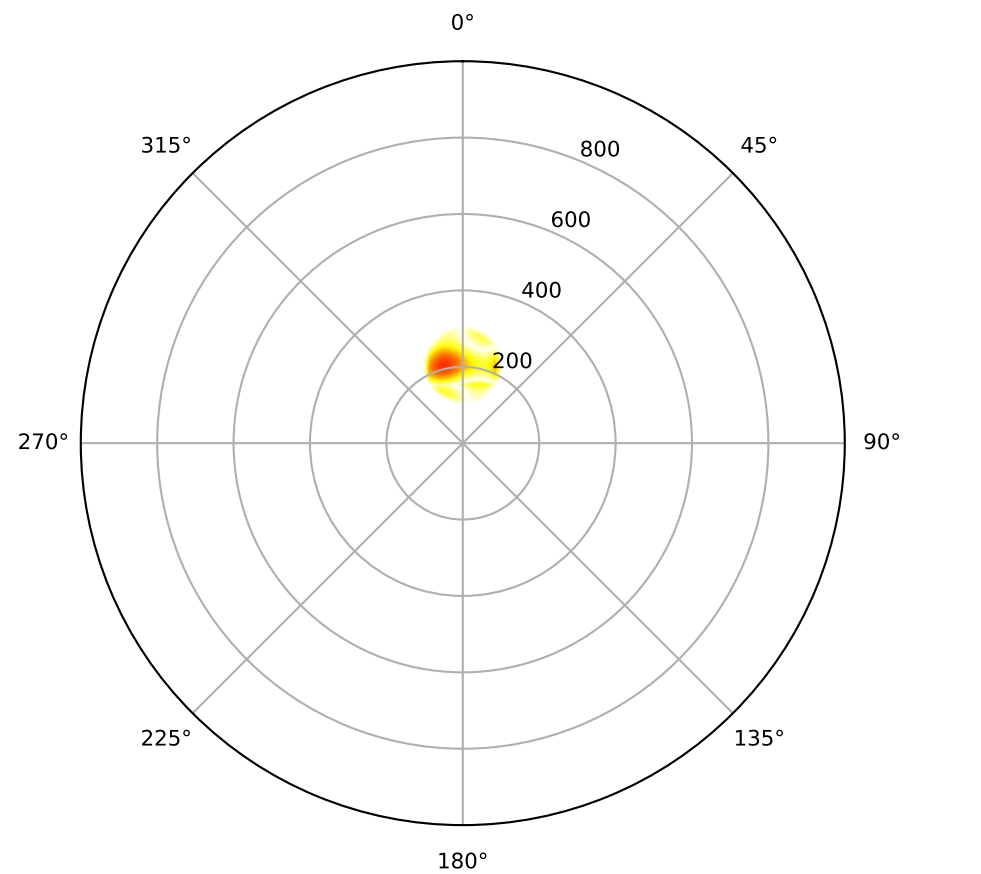
griddata MAE=1.2358
