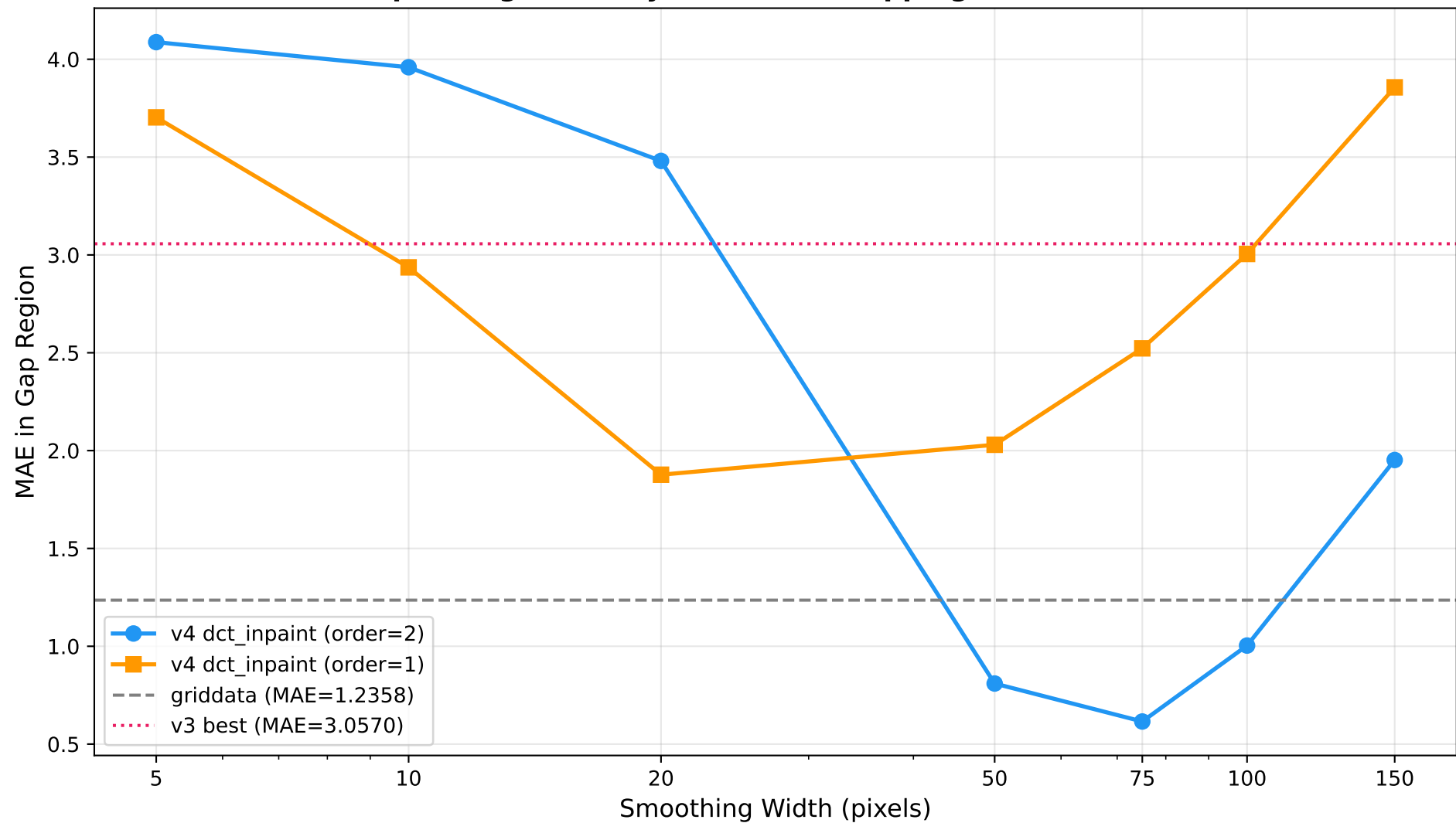
v4 Inpainting Accuracy vs Width (wrapping hole benchmark)
