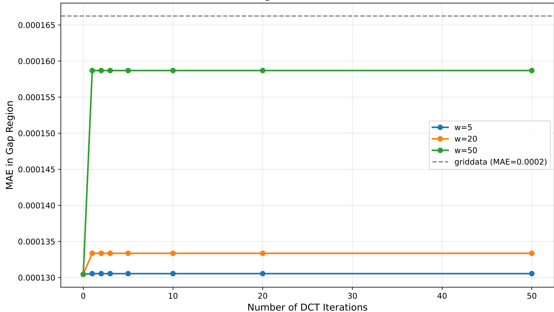
Iteration Convergence from Linear Initialization
