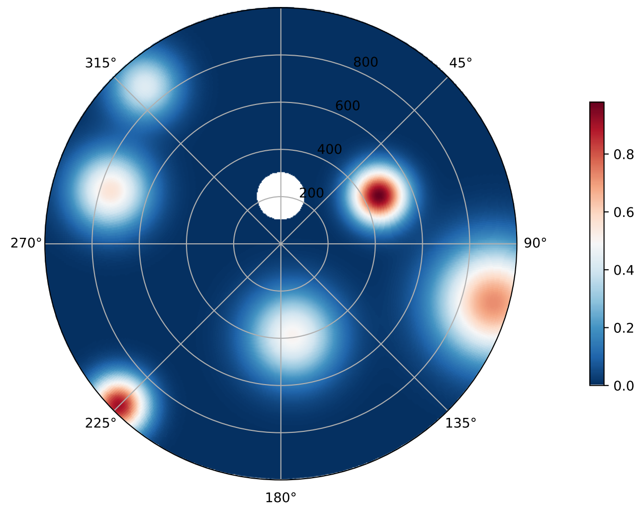
Griddata 0° (linear)
