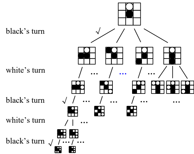
Fig. 14.5 Maximin decision of Tic-Tac-Toe.
