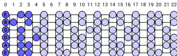
E Aeolian
