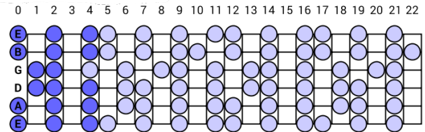
E Dorian
