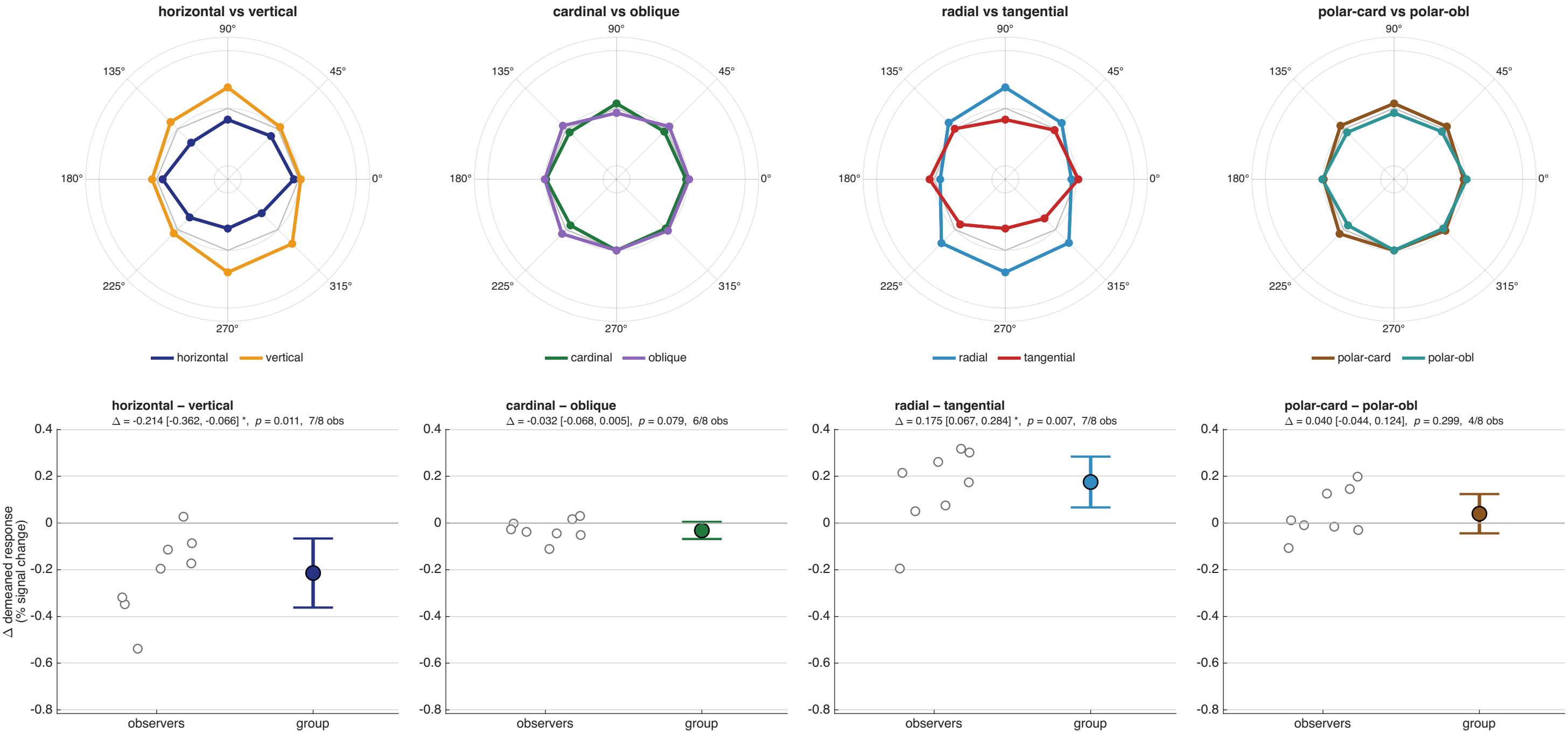
Figure 6, ALTERNATIVE ROUTE Polar gratings (da) | V1, 4-8° | n = 8 ROI route, eight polar-angle wedges, precision weighting | equal coverage at 45°, gain per observer × map, fit per observer then combined lines join the observed wedge means (this route fits no model); radius is the deviation from each vertex's mean over the four orientations
