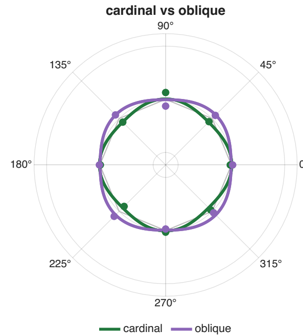
Figure 6, settled specification Polar gratings (da) | V1, 4-8° | n = 7 harmonic model, continuous \theta_V , equal weighting | equal coverage at 45°, gain per observer \times map, fit per observer then combined lines = fitted model (0.5°), markers = observed wedge means (45°); radius is the deviation from each vertex's mean over the four orientations
