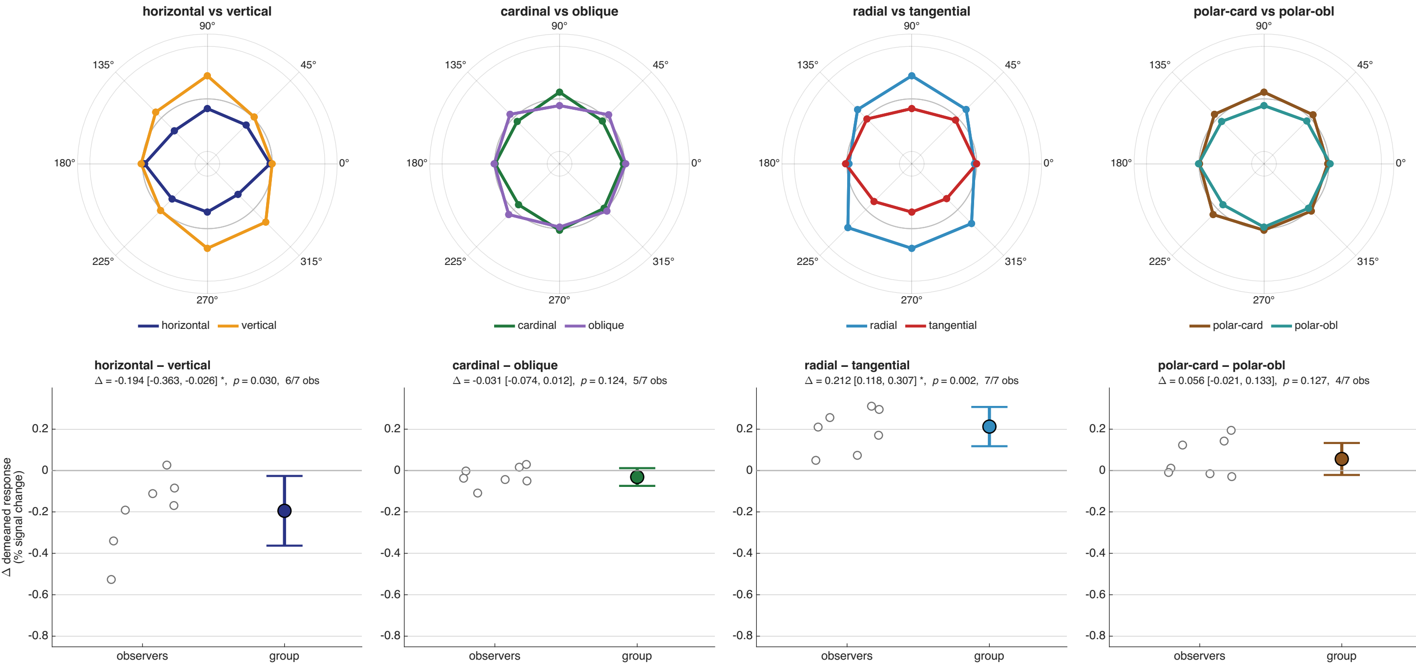
Figure 6, ALTERNATIVE ROUTE Polar gratings (da) | V1, 4-8° | n = 7 ROI route, eight polar-angle wedges, precision weighting | equal coverage at 45°, gain per observer × map, fit per observer then combined lines join the observed wedge means (this route fits no model); radius is the deviation from each vertex's mean over the four orientations
