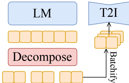
(c) Composition Prior ✓ Fidelity ✓
