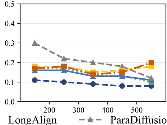
Character Location
