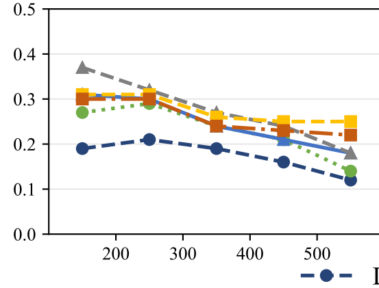
Character Presence
