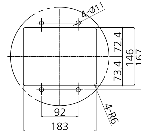
DETAIL A SCALE : 1.000
