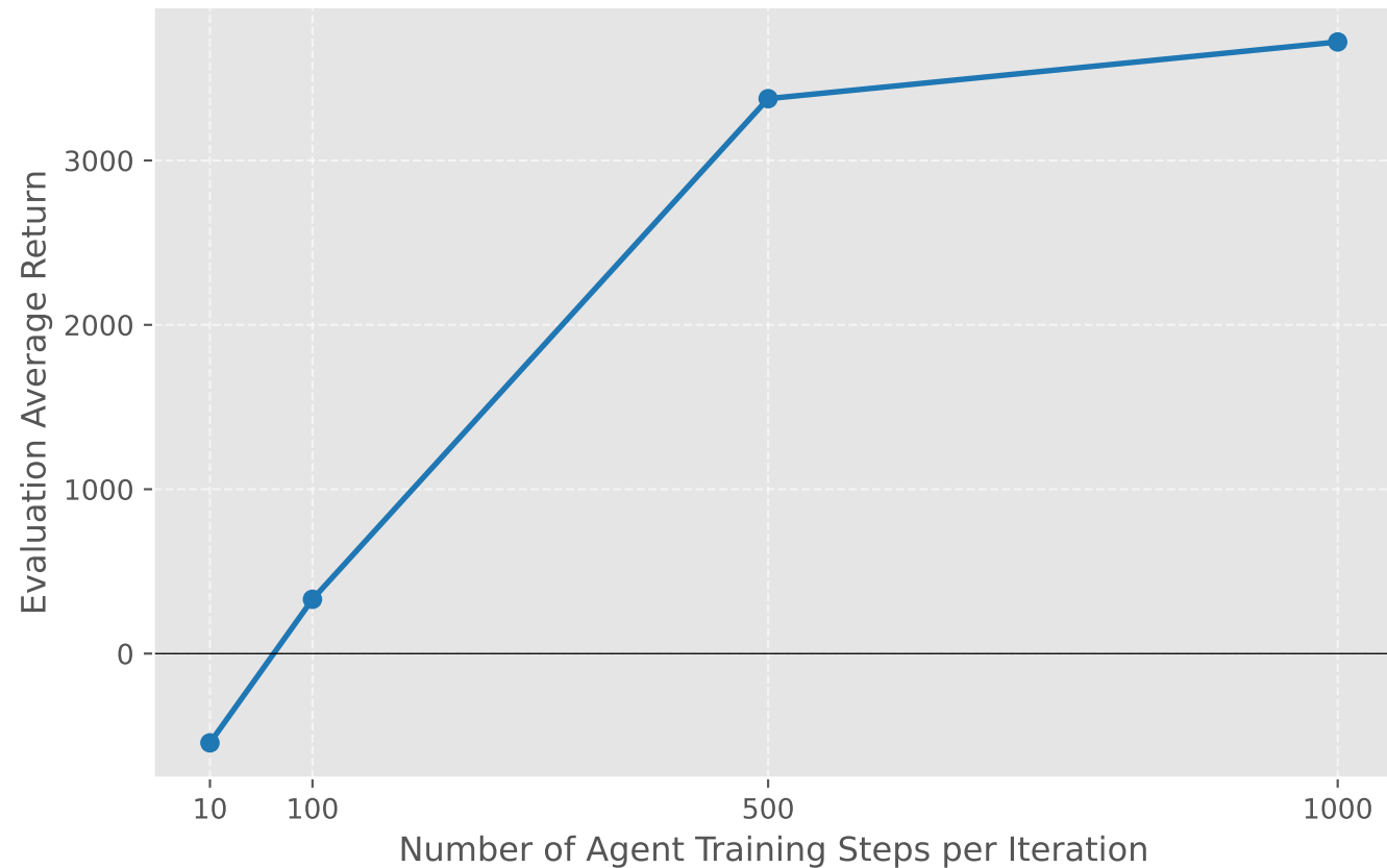
BC Performance vs. Training Steps (HalfCheetah-v4)
