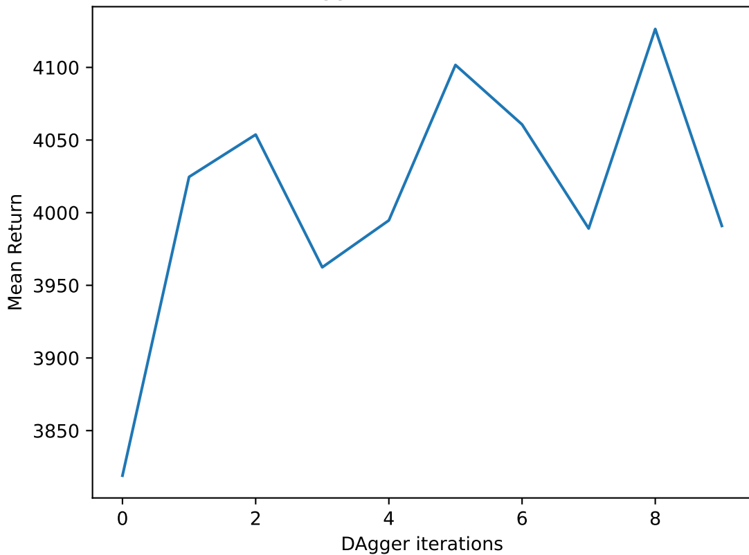
DAgger: HalfCheetah-v4
