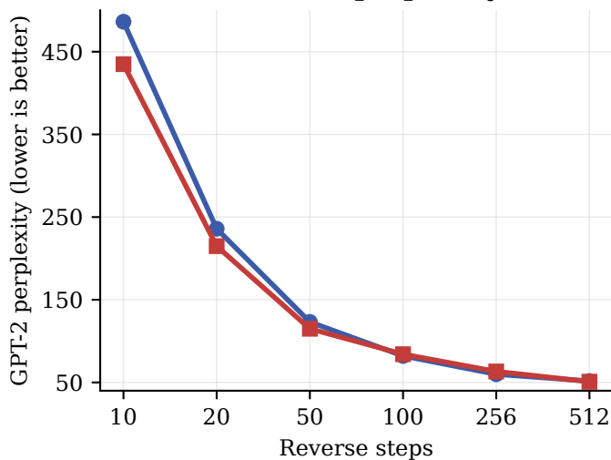
(c) SEDD perplexity
