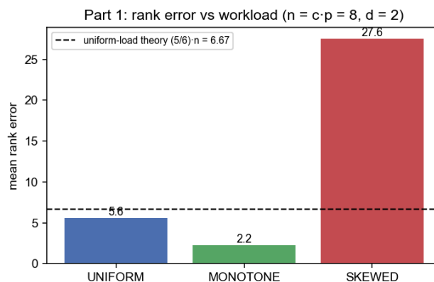
Figure 1. UNIFORM validates the harness against the closed form; MONOTONE (key order alone) is harmless; SKewed (non-uniform placement) blows the bound by ~4×
