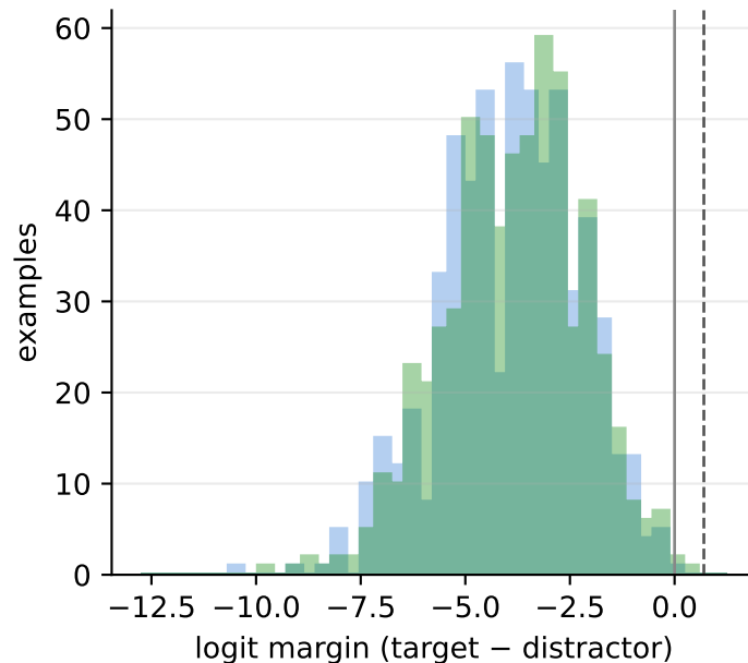
FAR margin distributions — all generated examples (dashed line: margin_thresh=0.7)
