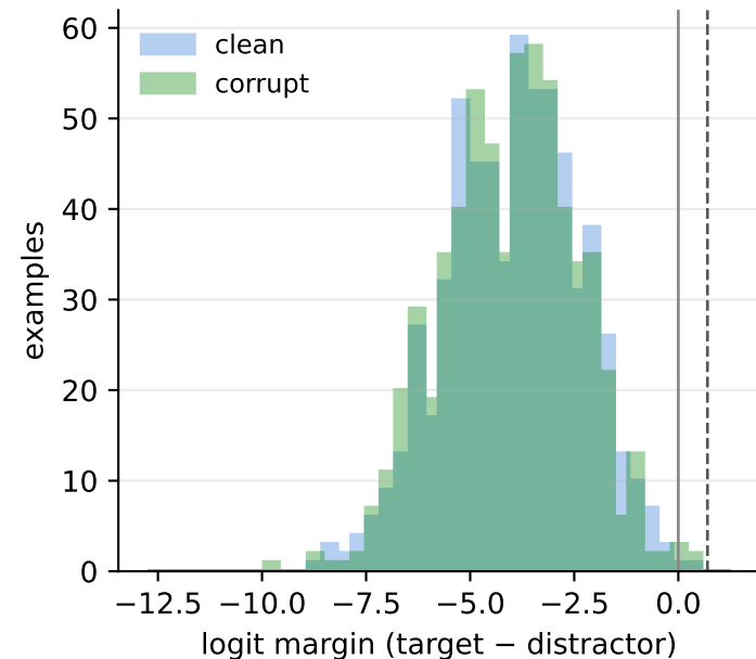
FAR margin distributions — all generated examples (dashed line: margin_thresh=0.7)
