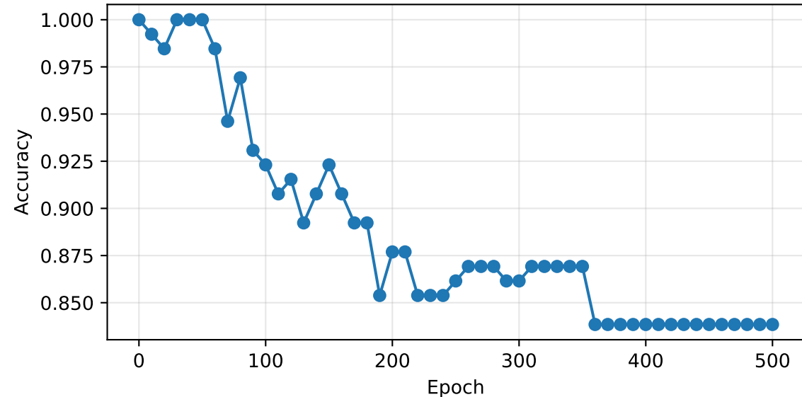
Faithfulness
