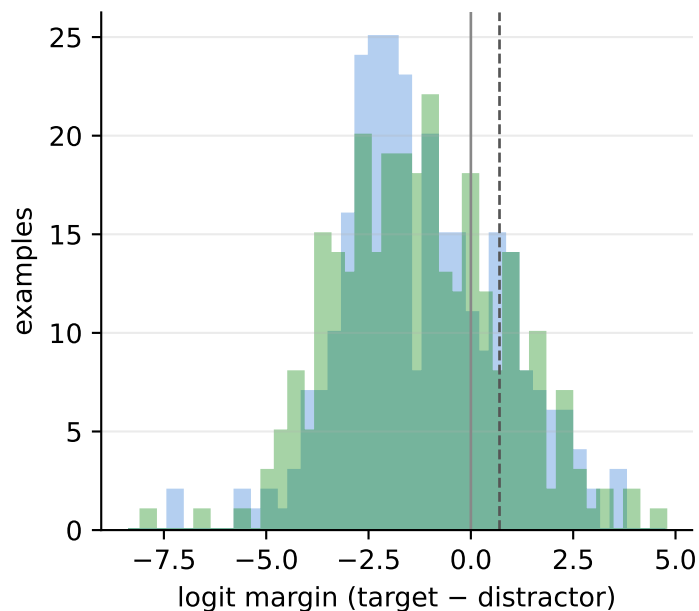
SER margin distributions — all generated examples (dashed line: margin_thresh=0.7)
