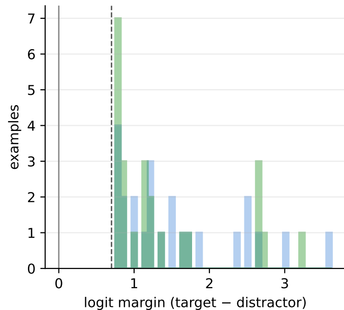
SER margin distributions — filter survivors only (dashed line: margin_thresh=0.7)
