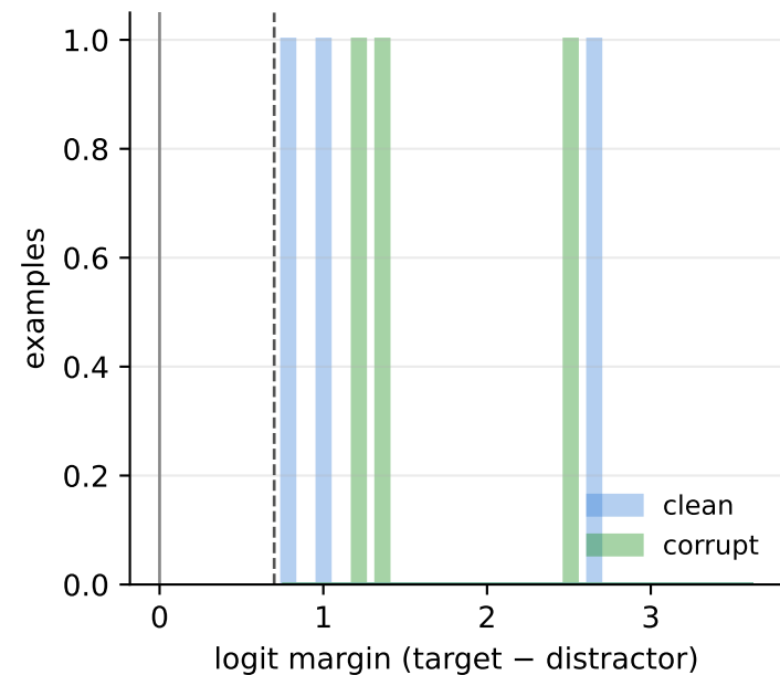
SER margin distributions — filter survivors only (dashed line: margin_thresh=0.7)
