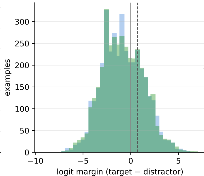
SDR margin distributions — all generated examples (dashed line: margin_thresh=0.7)
