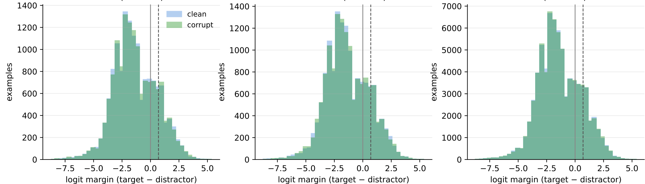
SER margin distributions — all generated examples (dashed line: margin_thresh=0.7)
