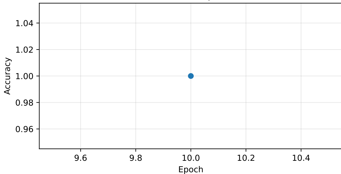
Faithfulness
