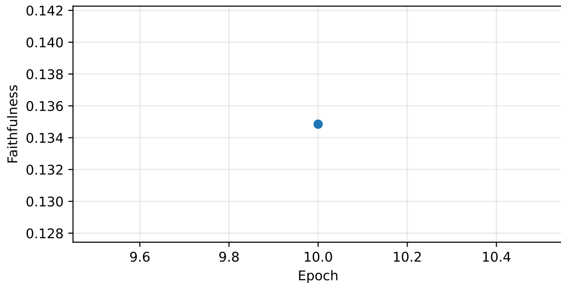
Faithfulness
