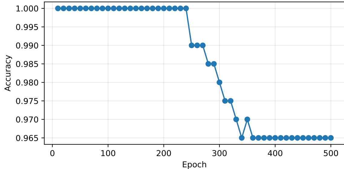
Faithfulness
