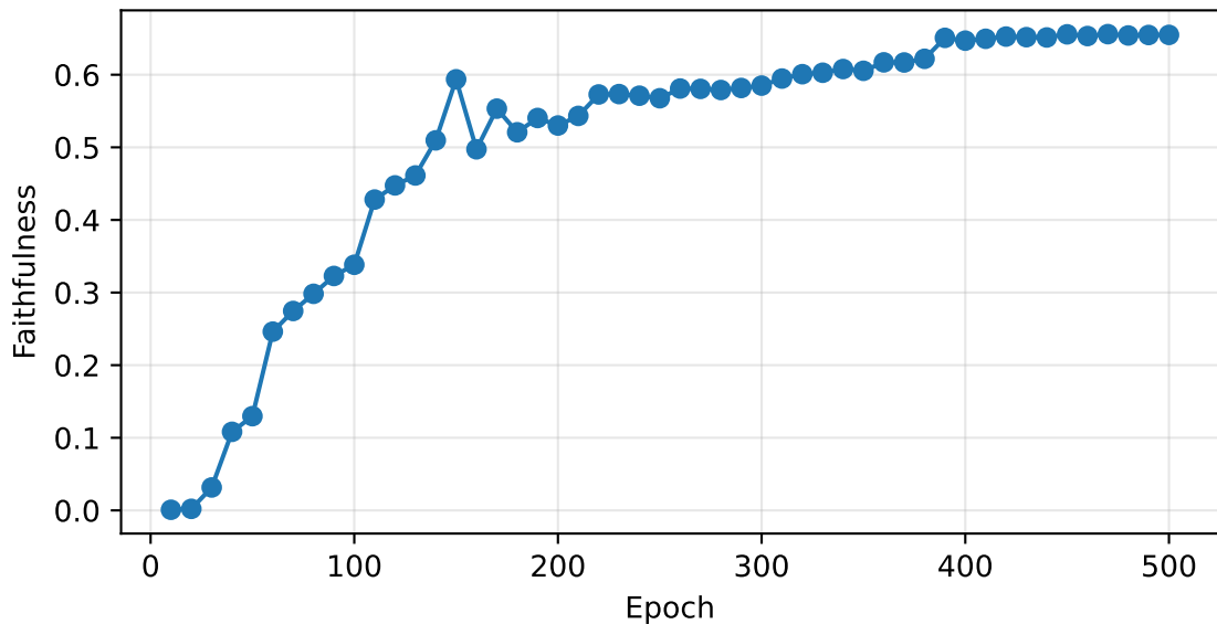
Faithfulness
