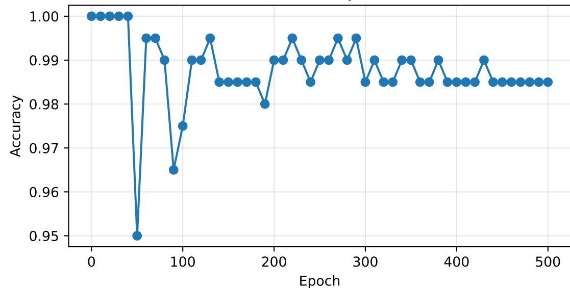
Faithfulness
