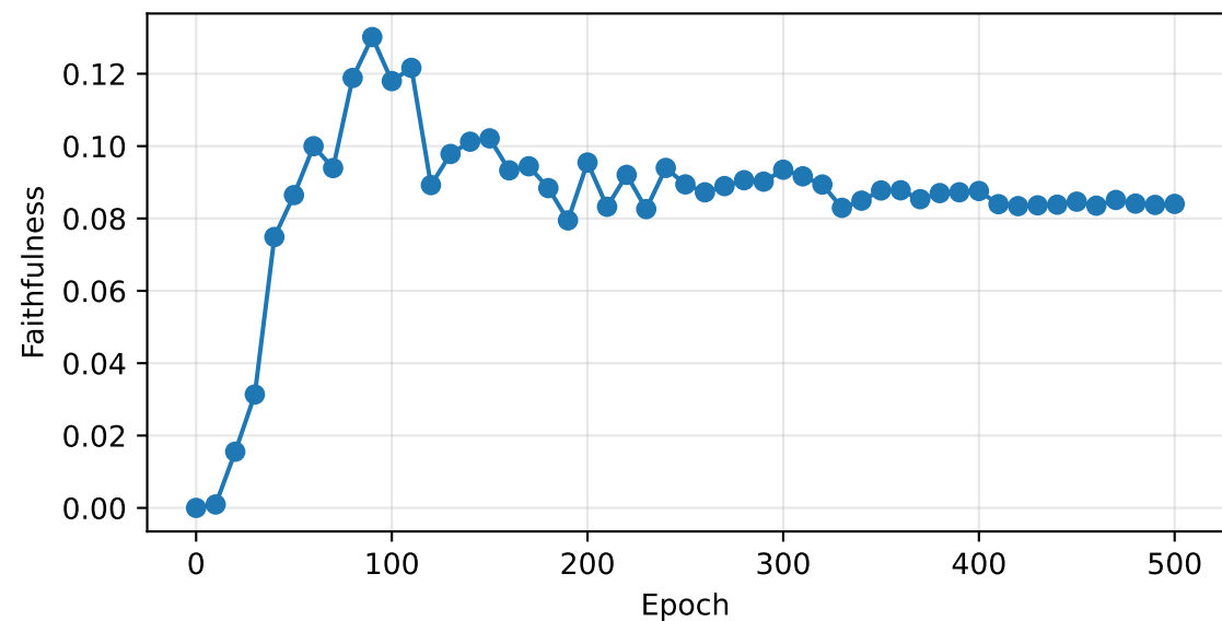
Faithfulness
