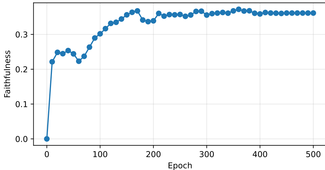
Faithfulness
