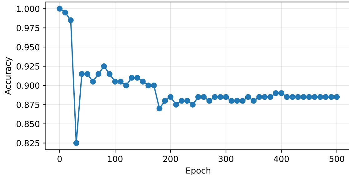
Faithfulness
