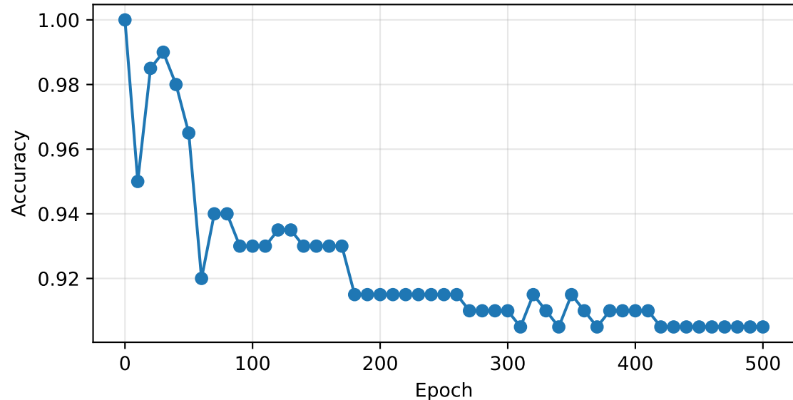
Faithfulness
