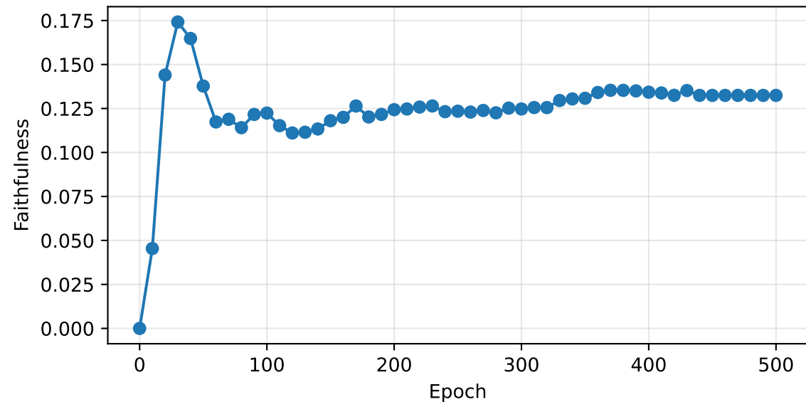
Faithfulness
