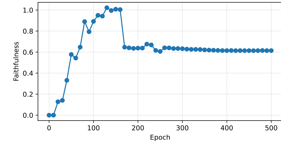
Faithfulness
