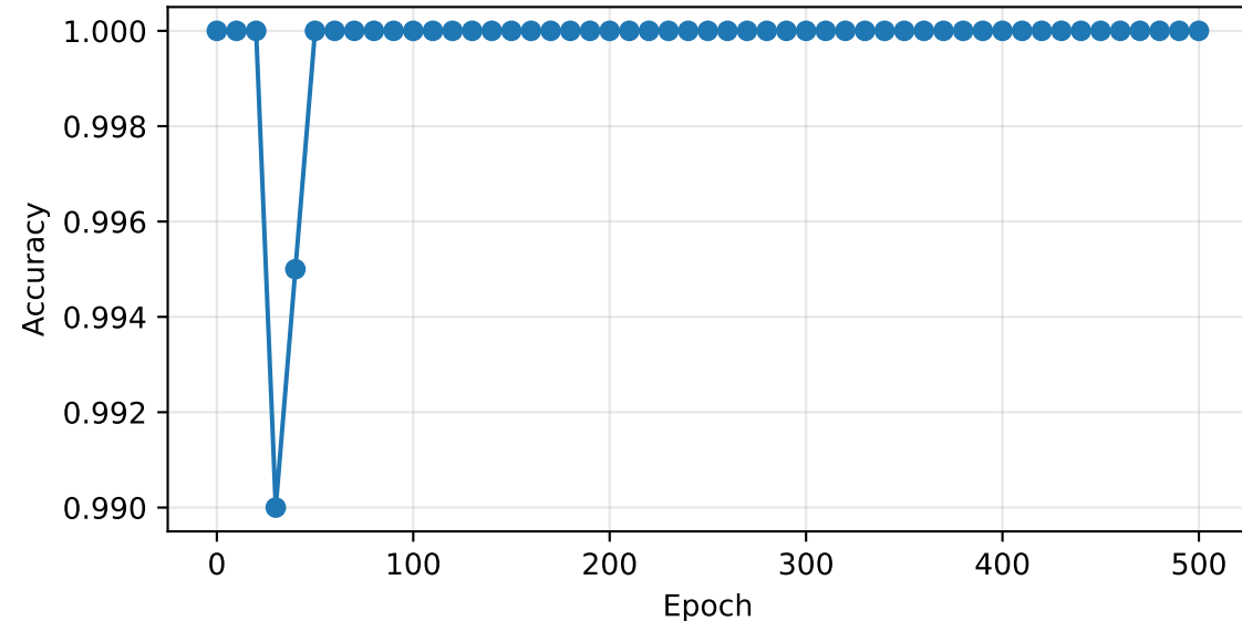
Faithfulness
