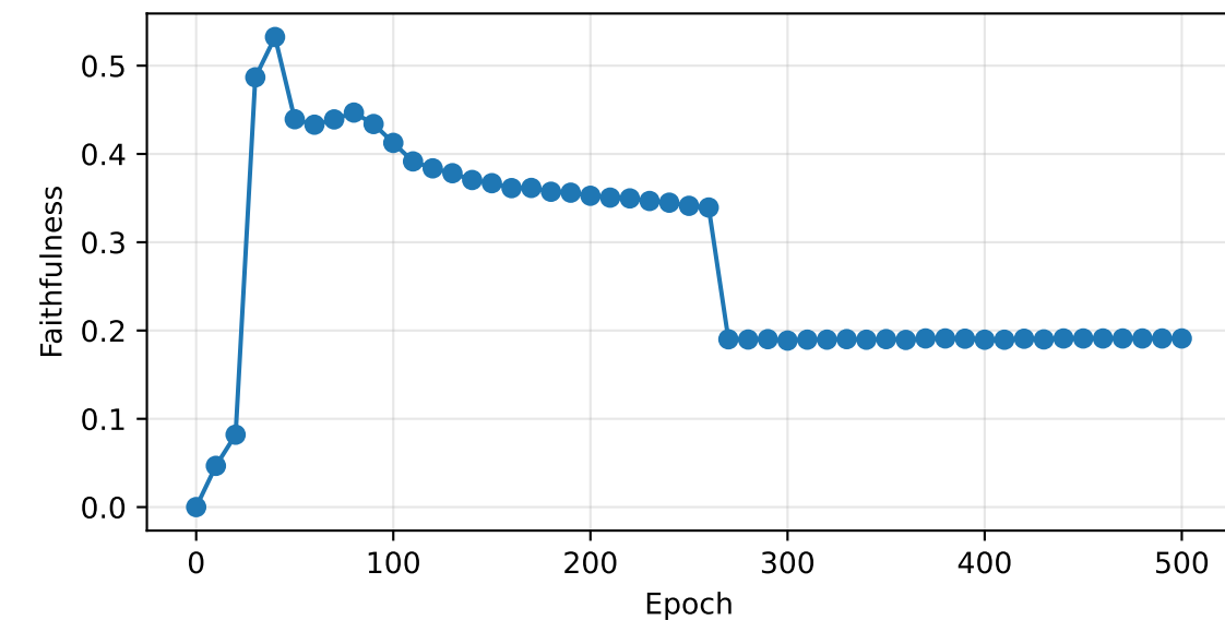
Faithfulness
