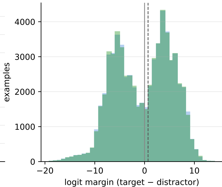
STD margin distributions — all generated examples (dashed line: margin_thresh=0.7)
