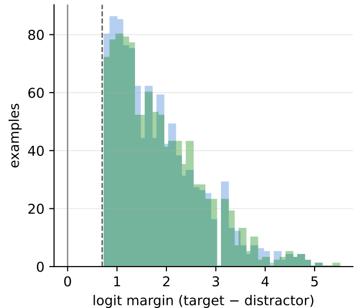
STD margin distributions — filter survivors only (dashed line: margin_thresh=0.7)
