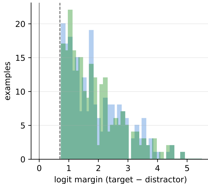
STD margin distributions — filter survivors only (dashed line: margin_thresh=0.7)
