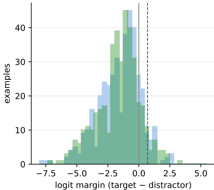
STD margin distributions (dashed line: margin_thresh=0.7)
