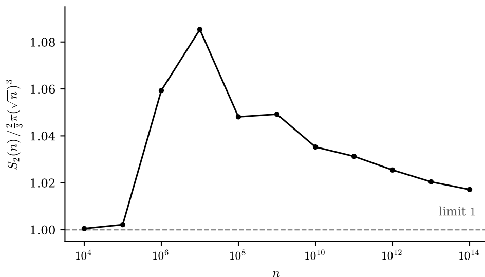
FIGURE 2. The quotient S_2(n)/\frac{2}{3}\pi(\sqrt{n})^3 against n , on a logarithmic n -axis, for n = 10^4, \dots, 10^{14} . Theorem 23 asserts that this tends to 1. It does, but only after rising to a maximum of 1.085 at n = 10^7 , and with a further slight rise between 10^8 and 10^9 ; at n = 10^{14} it is still 1.017. The two smallest values, at 10^4 and 10^5 , sit within 0.3% of 1 by coincidence rather than for any reason, which is a useful warning on its own. Values for n \leq 10^9 are from a least-prime-factor sieve, those beyond from an O(n^{3/4}) prime-counting recursion [28].
