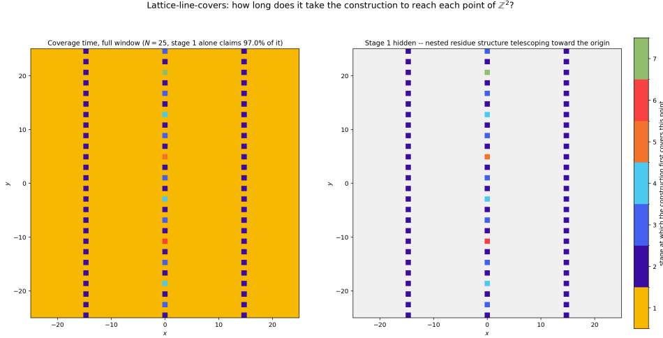
FIGURE 9. \text{stage}(u, v) over a 51 \times 51 window ( N = 25 ) of the run behind Figure 7. Left: the full window — stage 1 alone (gold) already claims 97.0% of it, since the first direction excludes only a single residue class. Right: stage 1 hidden, revealing that of the three residual columns visible on the left, only the one nearest the origin keeps recursing (through stages 3–7, telescoping inward as |y| grows), while the other two are fully resolved by stage 2 alone and never revisited — a direct consequence of z_k being enumerated by distance from the origin, so whichever residual region sits closest is exactly the one reopened next.
