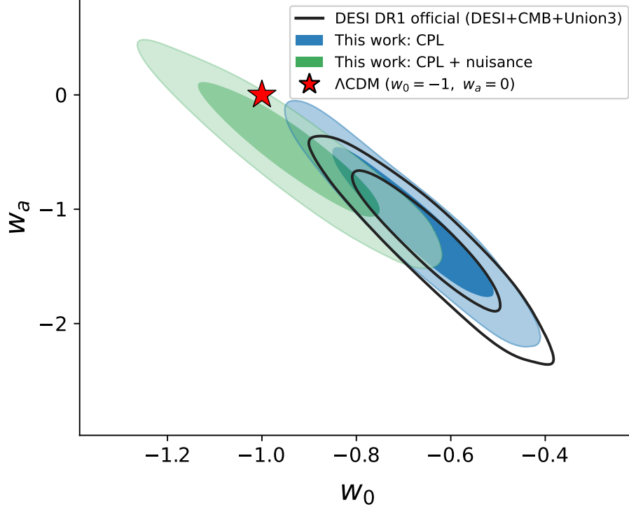
Figure 1: Full-likelihood joint cross-check in the w_0 - w_a plane. Black contours: DESI DR1 official w_0w_a CDM posterior (DESI+CMB+Union3, plik TT,TE,EE). Blue: this work’s CPL (NPIPE CamSpec); green: this work’s CPL+nuisance. Red star marks \Lambda CDM ( w_0 = -1 , w_a = 0 ). This work’s CPL reproduces the official DESI contour ( w_0 = -0.68 , w_a = -1.14 vs DESI w_0 = -0.64 , w_a = -1.30 ), the small offset being consistent with the different CMB likelihood choice; marginalizing the Union3 nuisance direction (green) shifts the posterior toward \Lambda CDM ( w_0 = -0.93 , w_a = -0.50 ), from \sim 2.4\sigma to \sim 1.6\sigma .
