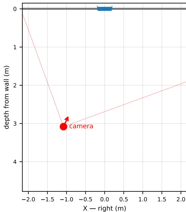
Floor plan — wall at top, board fixed, camera moves
