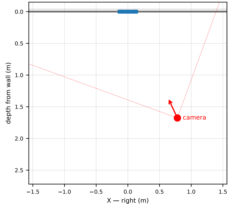
Floor plan — wall at top, board fixed, camera moves
