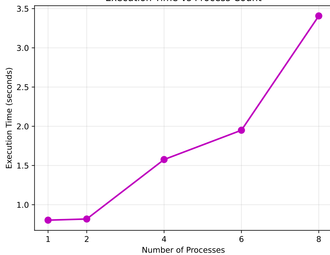
Execution Time vs Process Count
