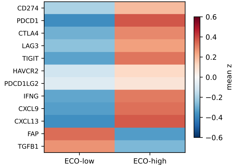
C. Immuno-stromal genes (IMvigor210)
