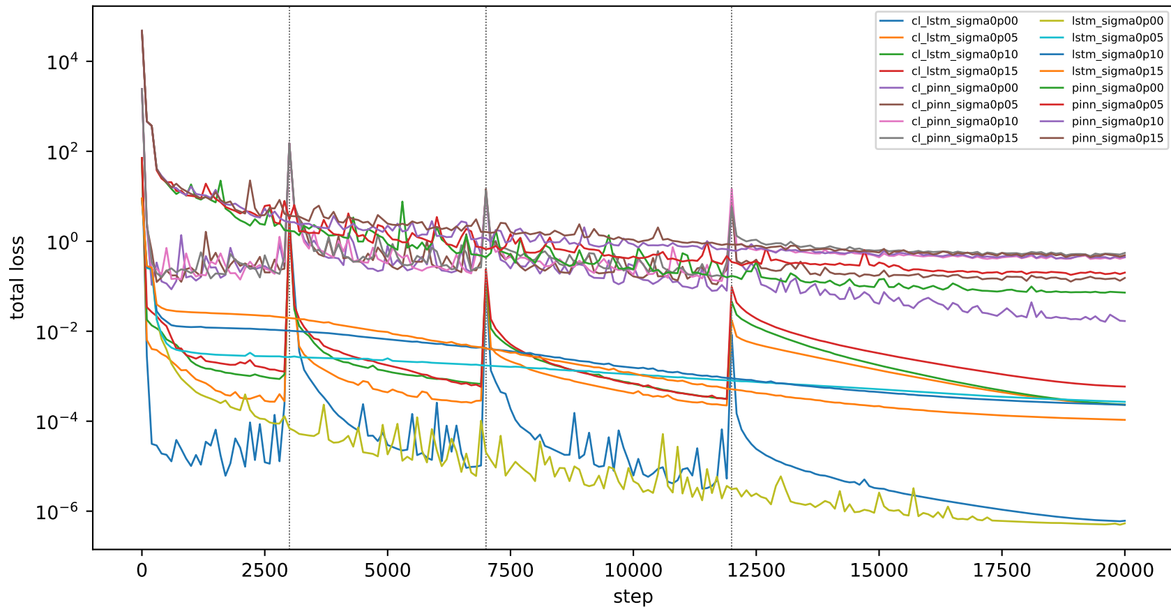
Training loss (dotted lines: curriculum stage boundaries)
