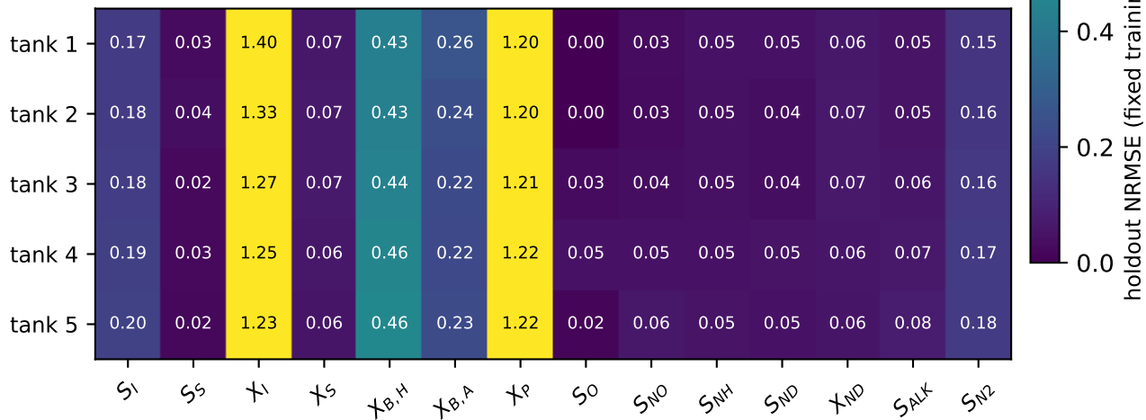
Single-stage PINN
