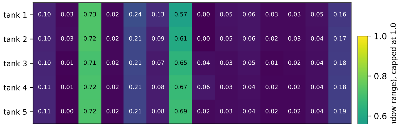
Curriculum PINN
