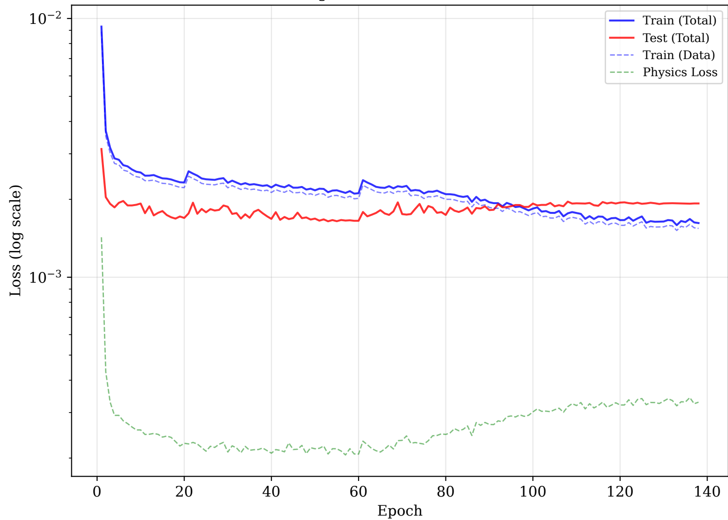
Training and Validation Loss Curve
