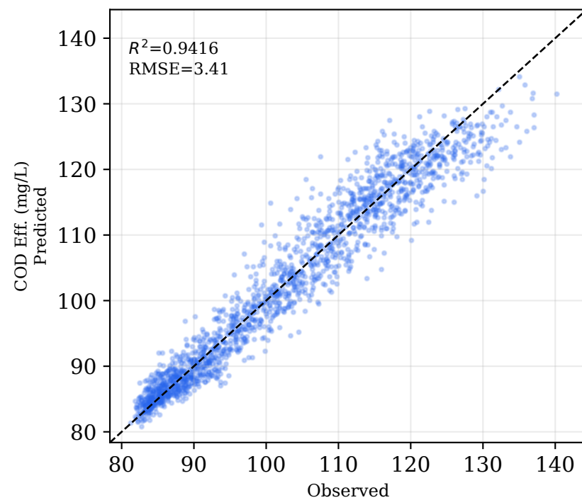
PG-LSTM
