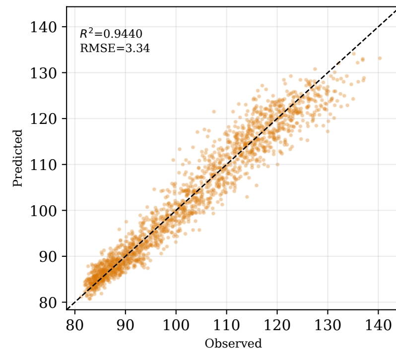
Vanilla LSTM
