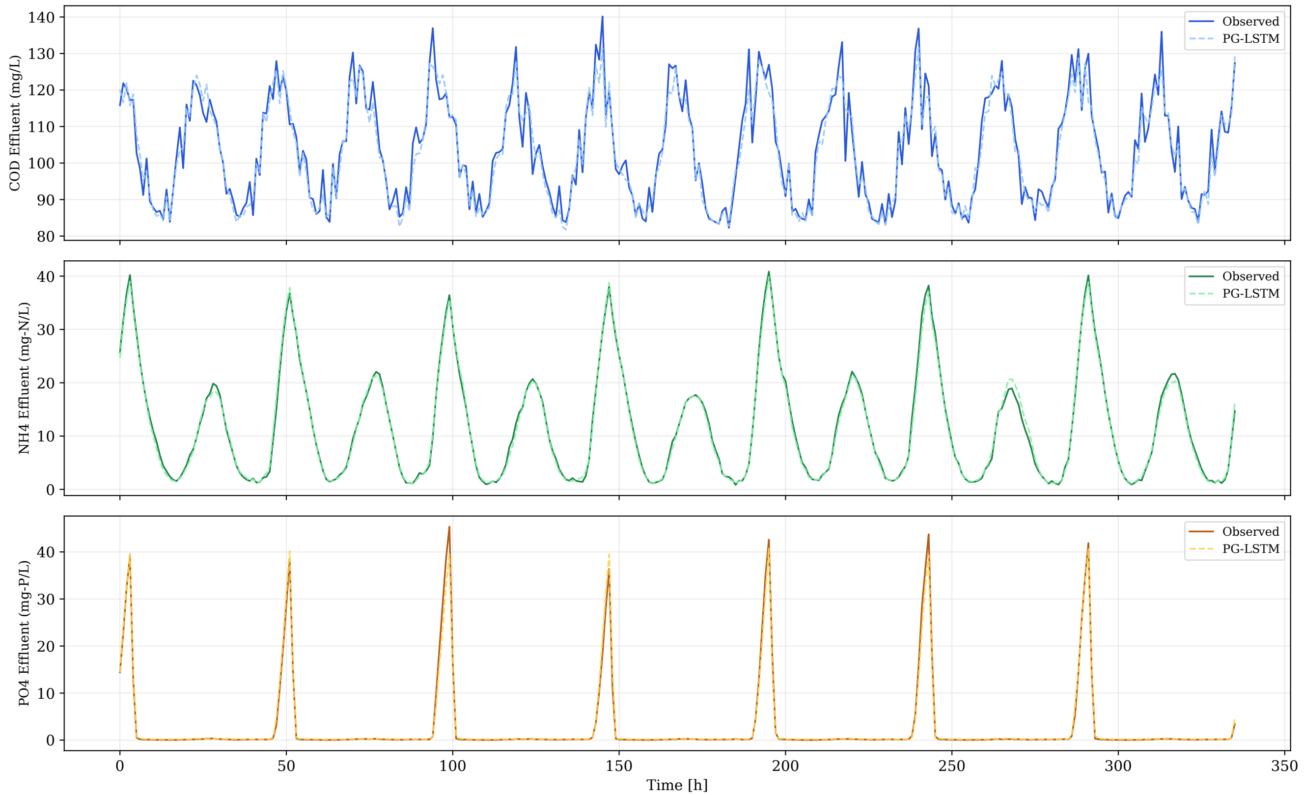
PG-LSTM: Observed vs. Predicted — First 14 Days (Test Set)
