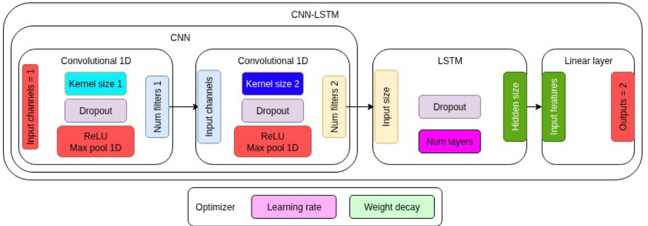
Figure 2: Structure of the implemented CNN-LSTM. All parts in red boxes are non-configurable, while boxes of all other colors contain parameters that were varied in a grid search. The dropout parameter is kept the same in all layers, in the interest of reducing the number of configurations searched.
