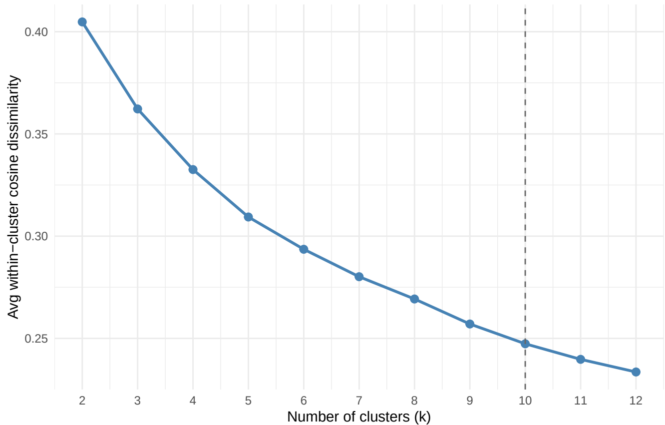
Elbow – spherical k-means dashed = silhouette-optimal k (10)
