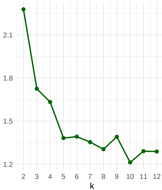
Davies-Bouldin spherical (lower better)
