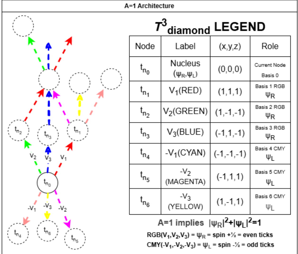
Figure 1: The \mathcal{T}^3_\diamond lattice architecture. The nucleus node t_{n_0} carries both Dirac spinor components ( \psi_R, \psi_L ). RGB basis vectors constitute the right-handed sublattice ( \psi_R , spin +1/2 , even ticks) and CMY basis vectors the left-handed sublattice ( \psi_L , spin -1/2 , odd ticks). The \mathcal{A}=1 constraint requires |\psi_R|^2 + |\psi_L|^2 = 1 .
